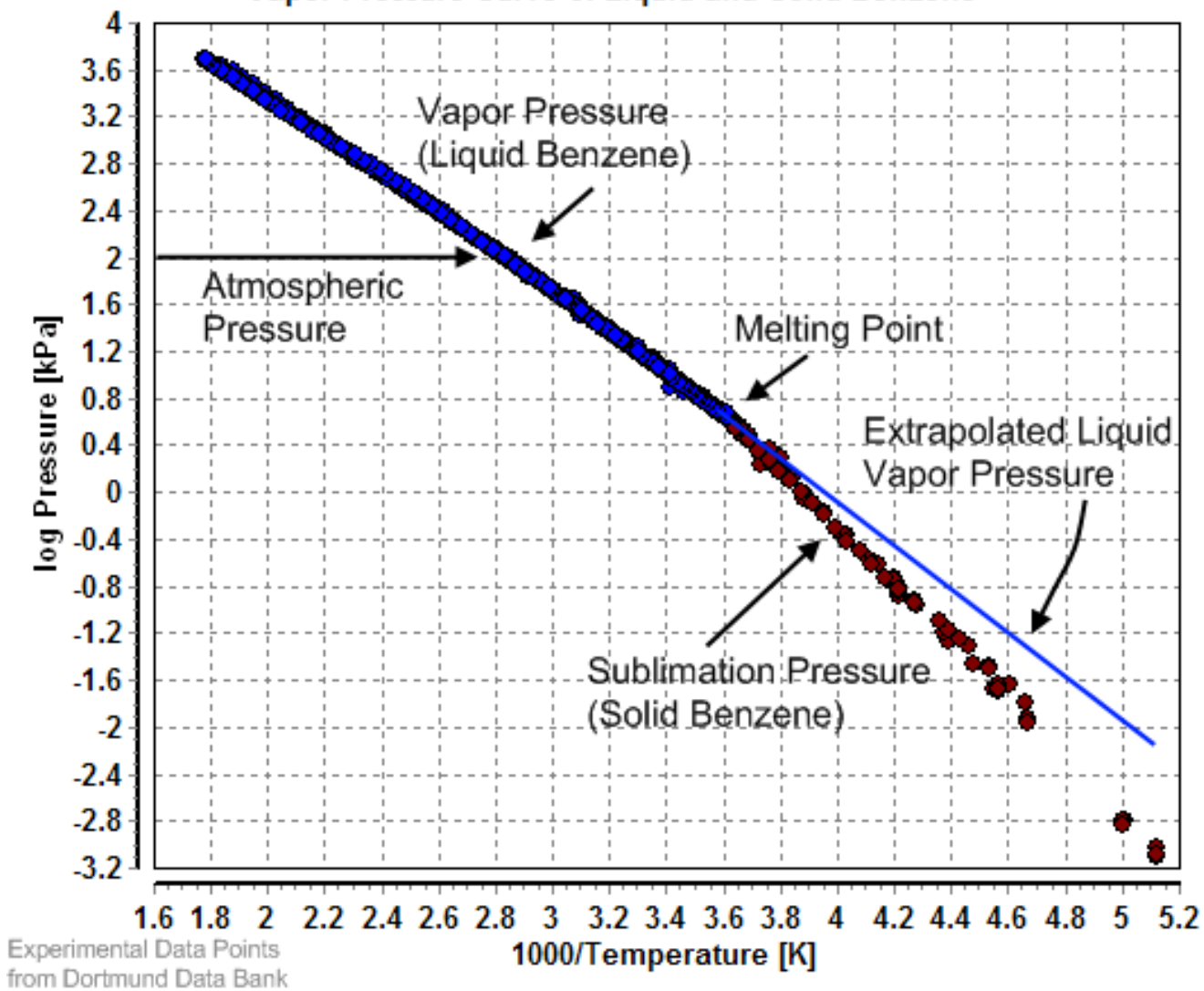
Vapor Pressure Curve of Liquid and Solid Benzene
